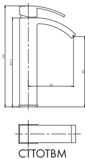
TORINO TALL BASIN MIXER
